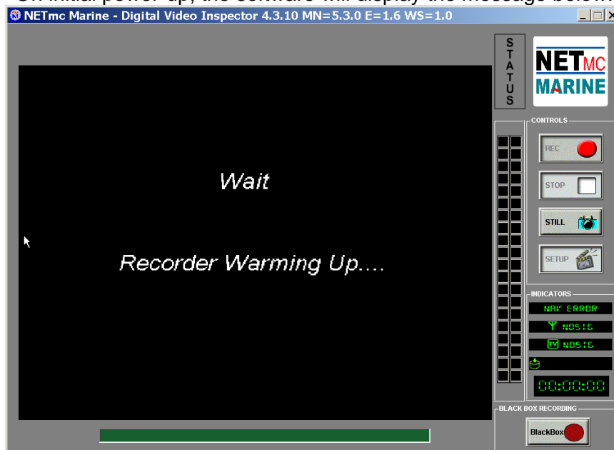
Splash screen
